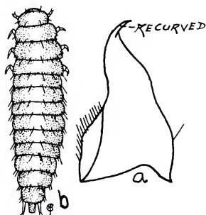
Fig. 192. a, Mandible; b, Platypsillus castoris Rits.
